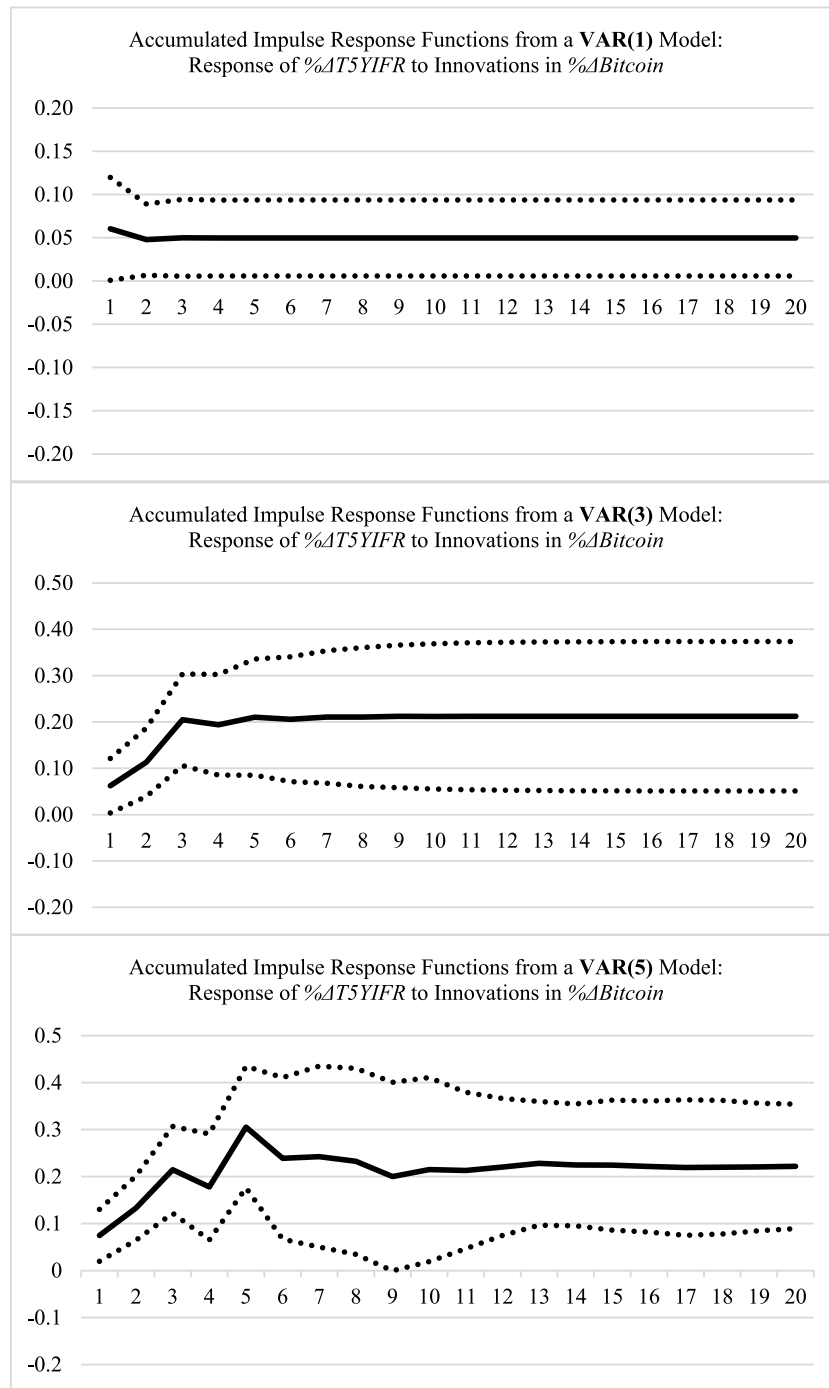
Fig. 1. The figure reports the accumulated impulse response functions from estimating VAR(1), VAR(3), and VAR(5) processes (i.e., one lag, three lags, and five lags) where %ΔT5YIFR and %ΔBitcoin are treated endogenously. The response of %ΔT5YIFR is plotted in response to a one-standard-deviation exogenous shock to %ΔBitcoin. The solid line represents the IRF while the dotted lines represent the upper (two-standard deviation) bound and the lower (two-standard deviation) bound.
